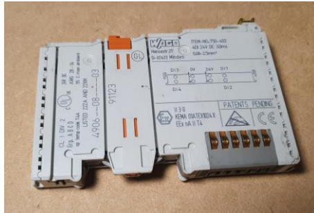
WAGO 750-402
