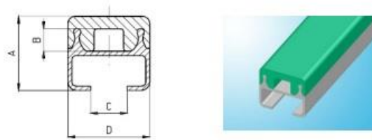
Aluminium profile with a flat guide GTCL3000 e 6000
