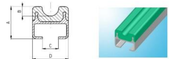
Aluminium profiles with a guide GTC polyethylene under round belt L3000 e 6000
